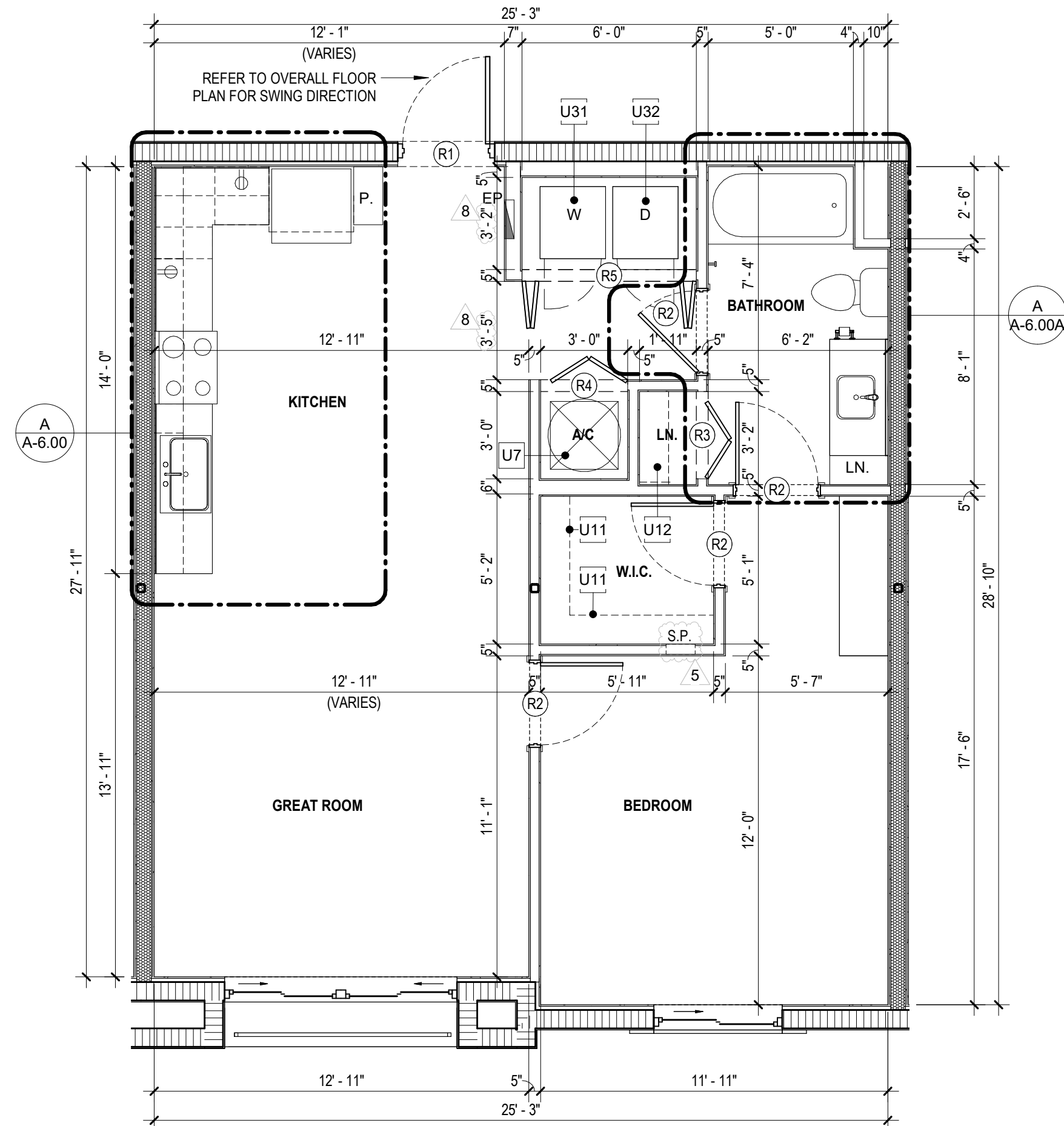
UNIT A1 TYP. FLOOR PLAN
