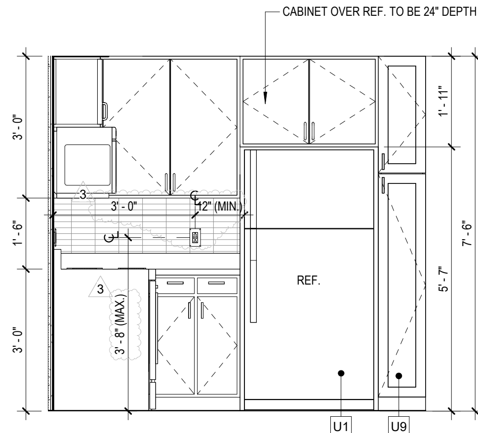
UNIT A1 KITCHEN EL.
