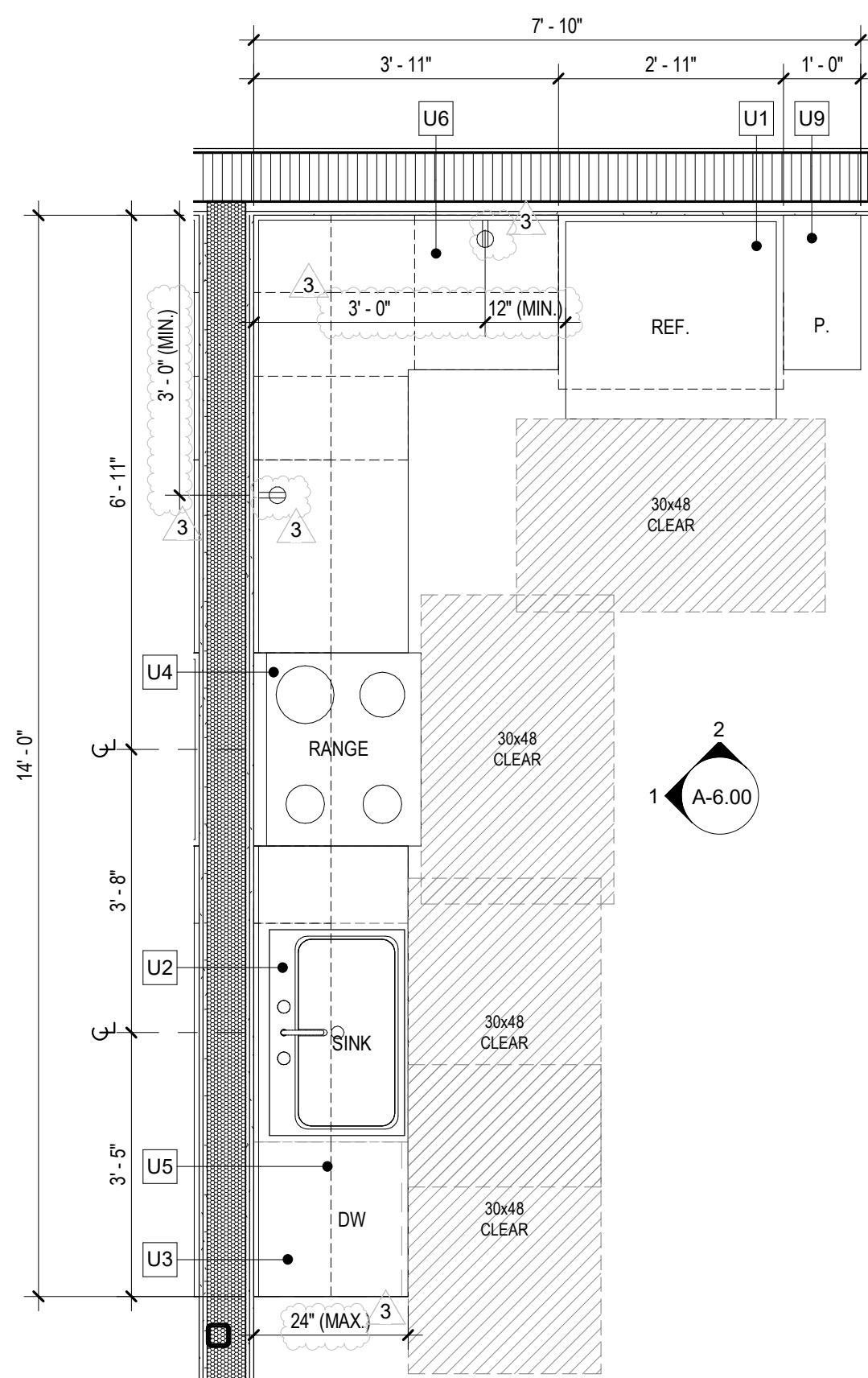
UNIT A1 KITCHEN PLAN
