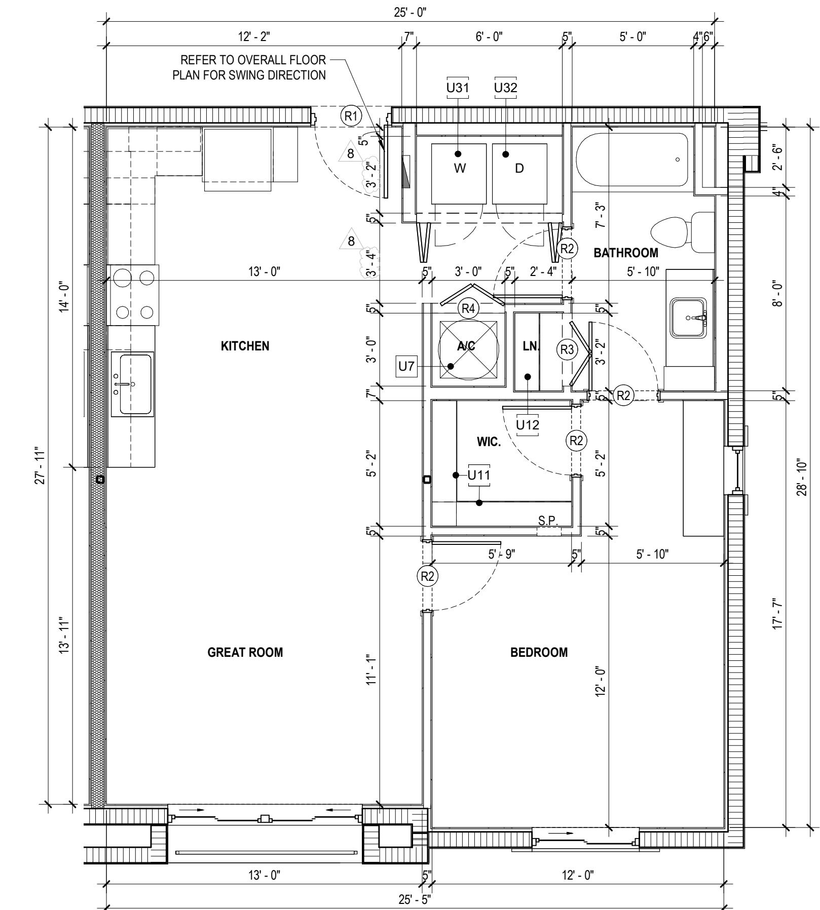
UNIT A1 (CORNER CONDITION) FLOOR PLAN
