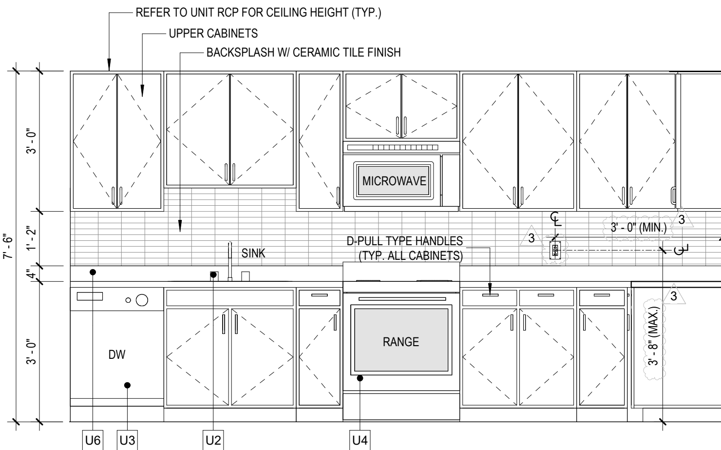
UNIT A1 KITCHEN EL.
